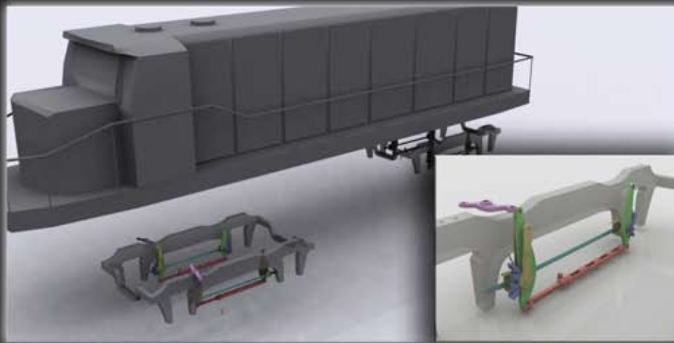
Truck components including brake rigging parts
